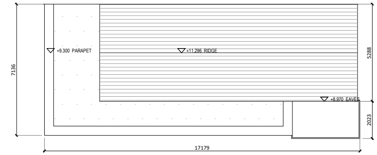
Roof Level 1:200
