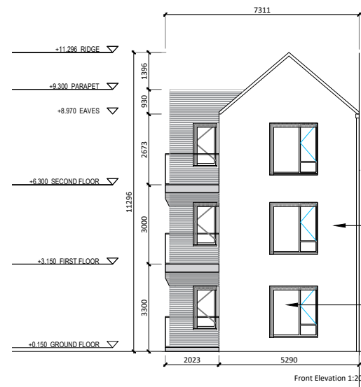
Front Elevation 1:200
