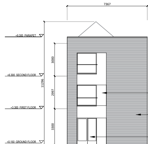
Rear Elevation 1:200
